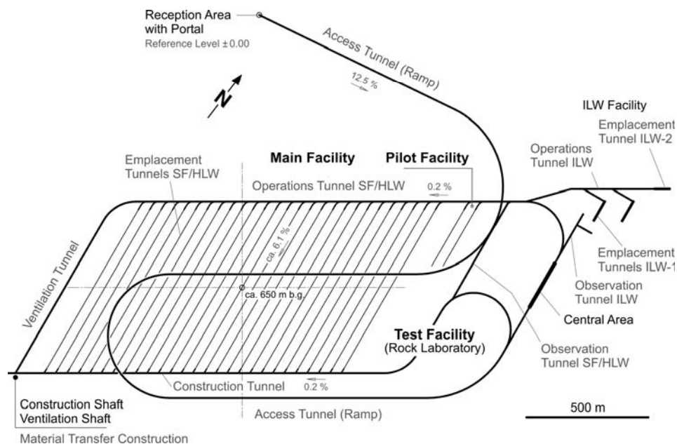
Figure 2: Co-location of HLW/SF and ILW facilities
