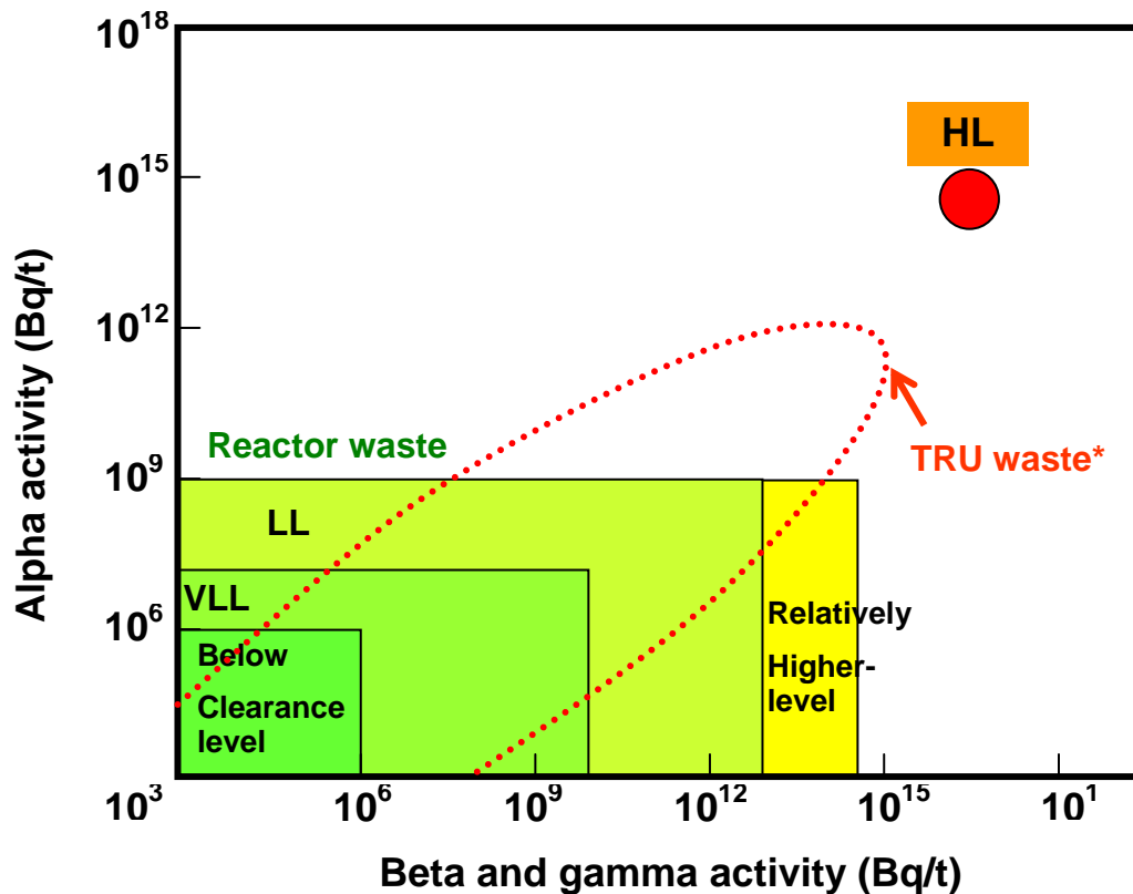
Figure 1. TRU waste categorisation in Japan.
